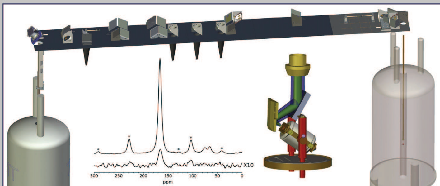
A DNP enhanced MAS NMR spectrometer which uses quasi-optic microwave transmission and a beam focussed into the rotor is described. It gives high-resolution spectra of solids with enhancements of up to x60.
